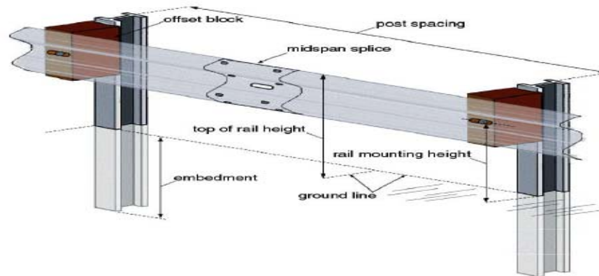
Figure 1: Use of midspan splices and offset blocks in a MGS (Ochoa, C & Ochoa, T, 2011).
