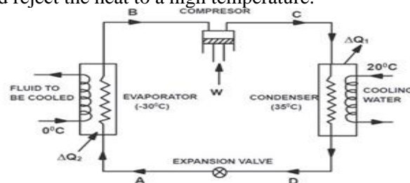
Fig 1: Vapour Compression Cycle.
